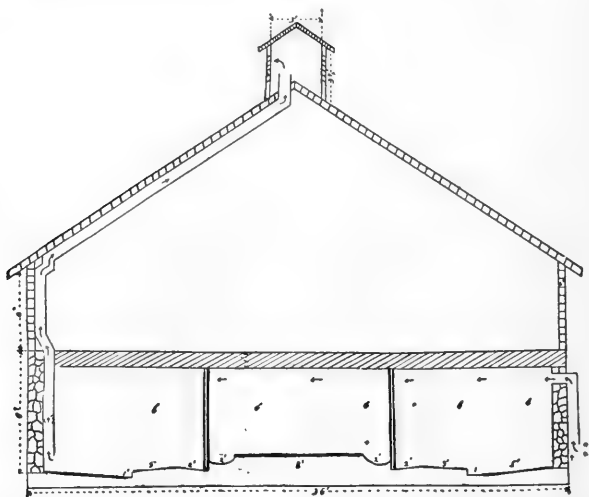
FIG. 215.—King system of ventilation for dairy barns. The air outlet should start near the floor and extend through the roof. The inlet for air into the stable is near the ceiling, but should start outside well above the ground. Windows are for light, not for ventilation, when the King system is in use.
